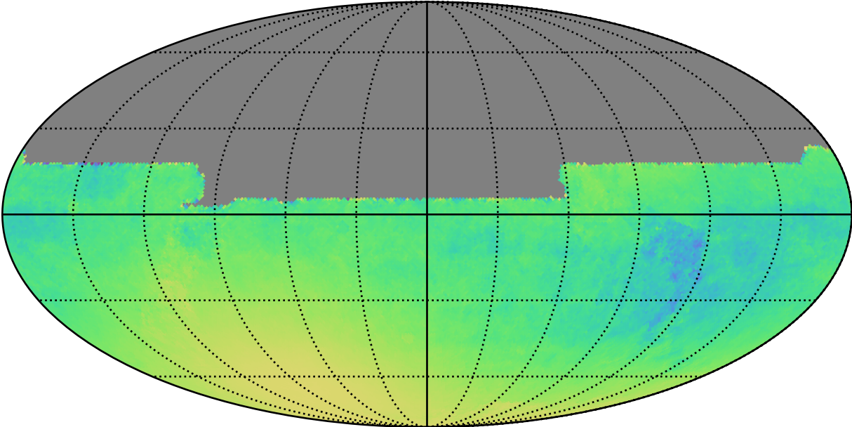
weather_cloudso35v3.4_10yrs All sky y band only: Normalized Parallax Uncert @ 21.3
