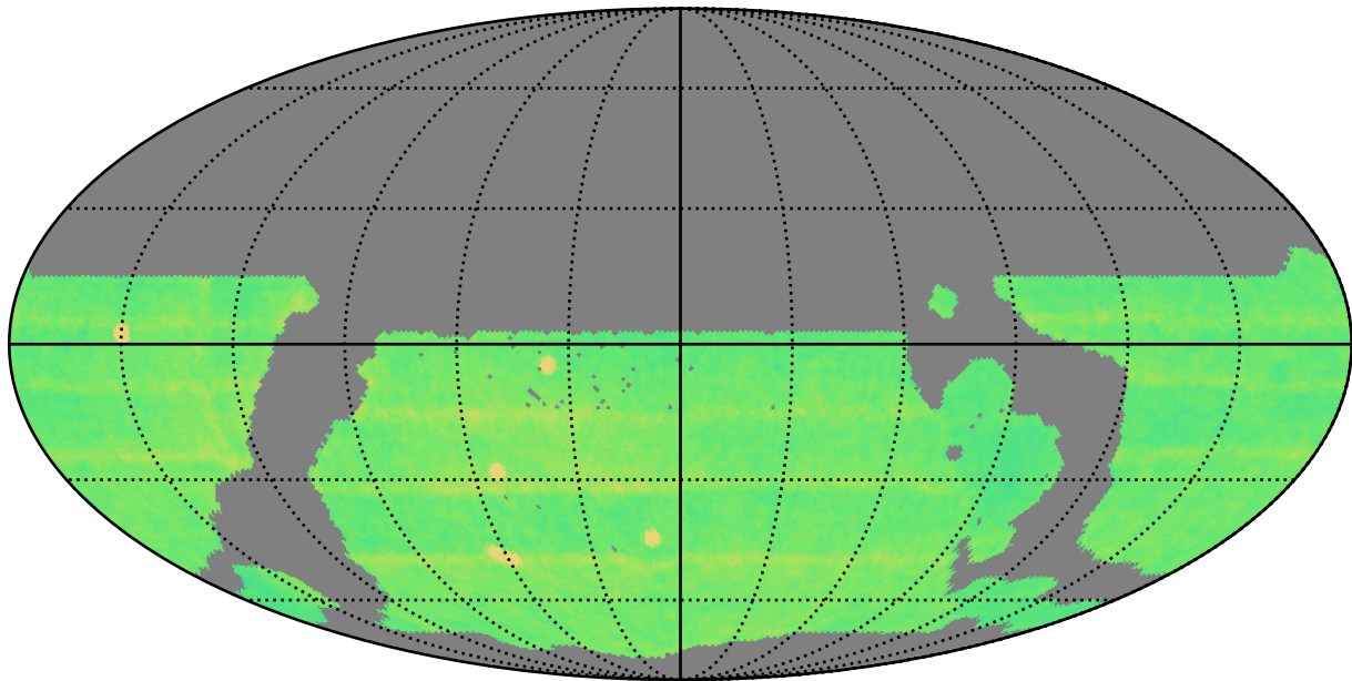
weather_cloudso35v3.4_10yrs WFD all bands: N Unique Nights
