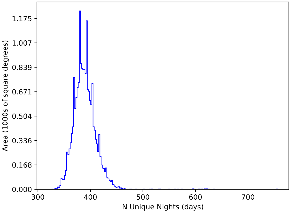
weather_cloudso35v3.4_10yrs WFD all bands: N Unique Nights
