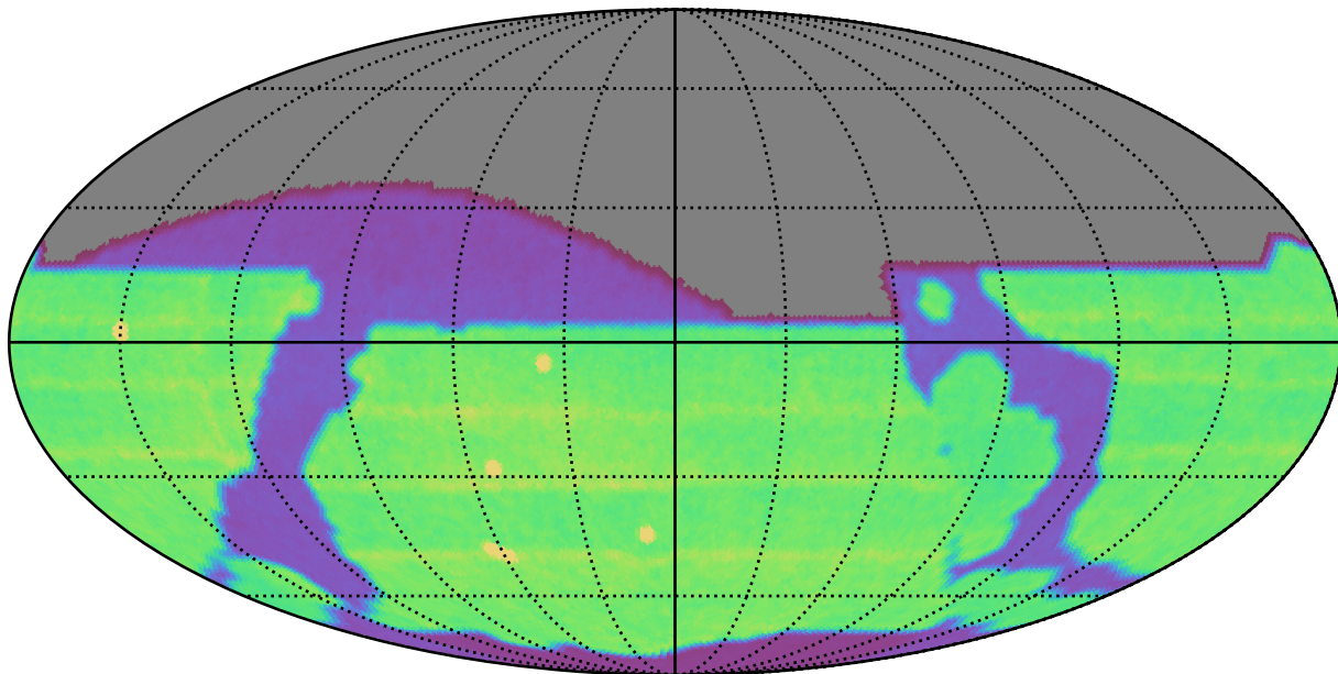
weather_cloudso35v3.4_10yrs All sky all bands: N Unique Nights
