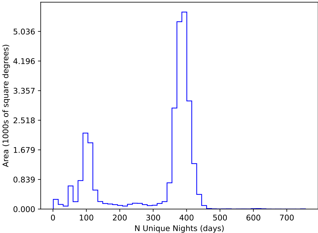
weather_cloudso35v3.4_10yrs All sky all bands: N Unique Nights
