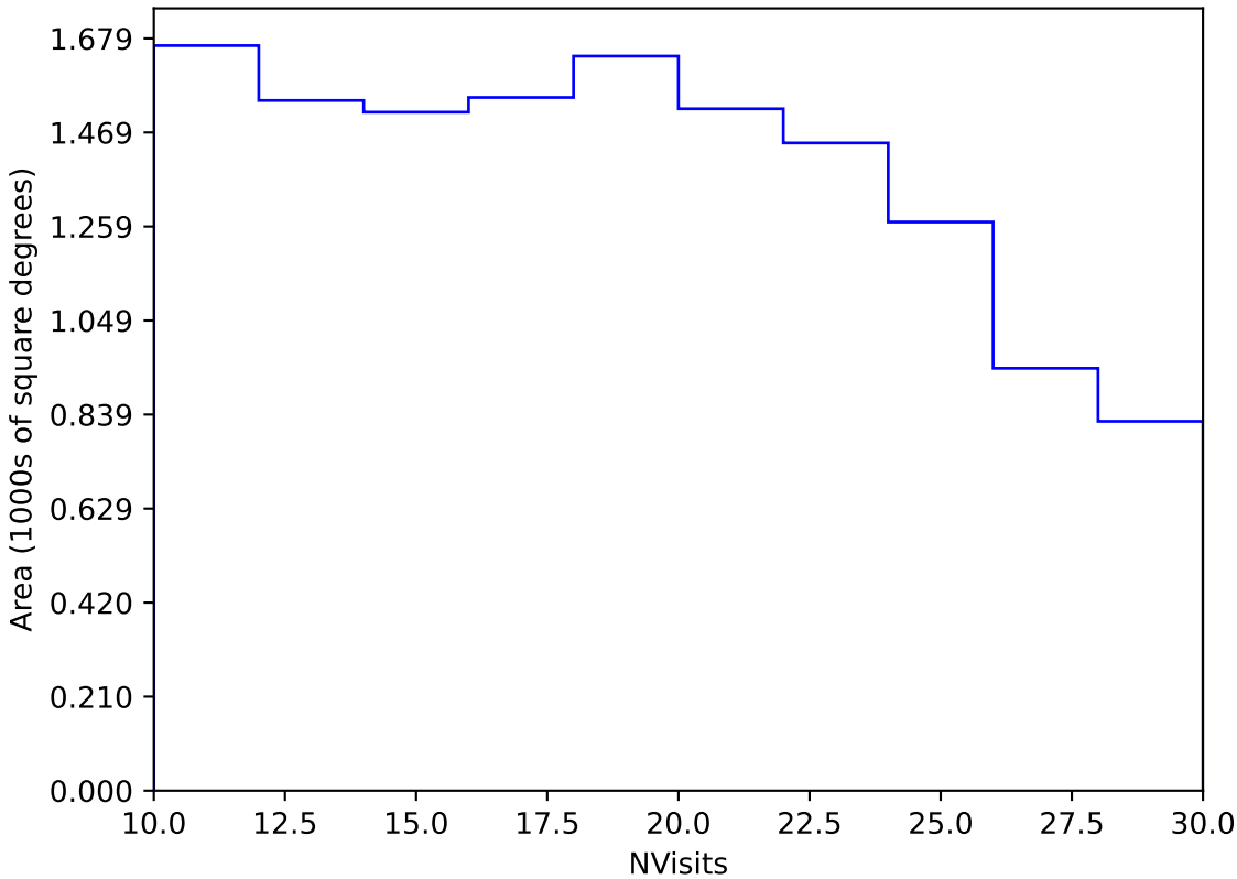
weather_cloudso35v3.4_10yrs Yr 3-4 y band: NVisits
