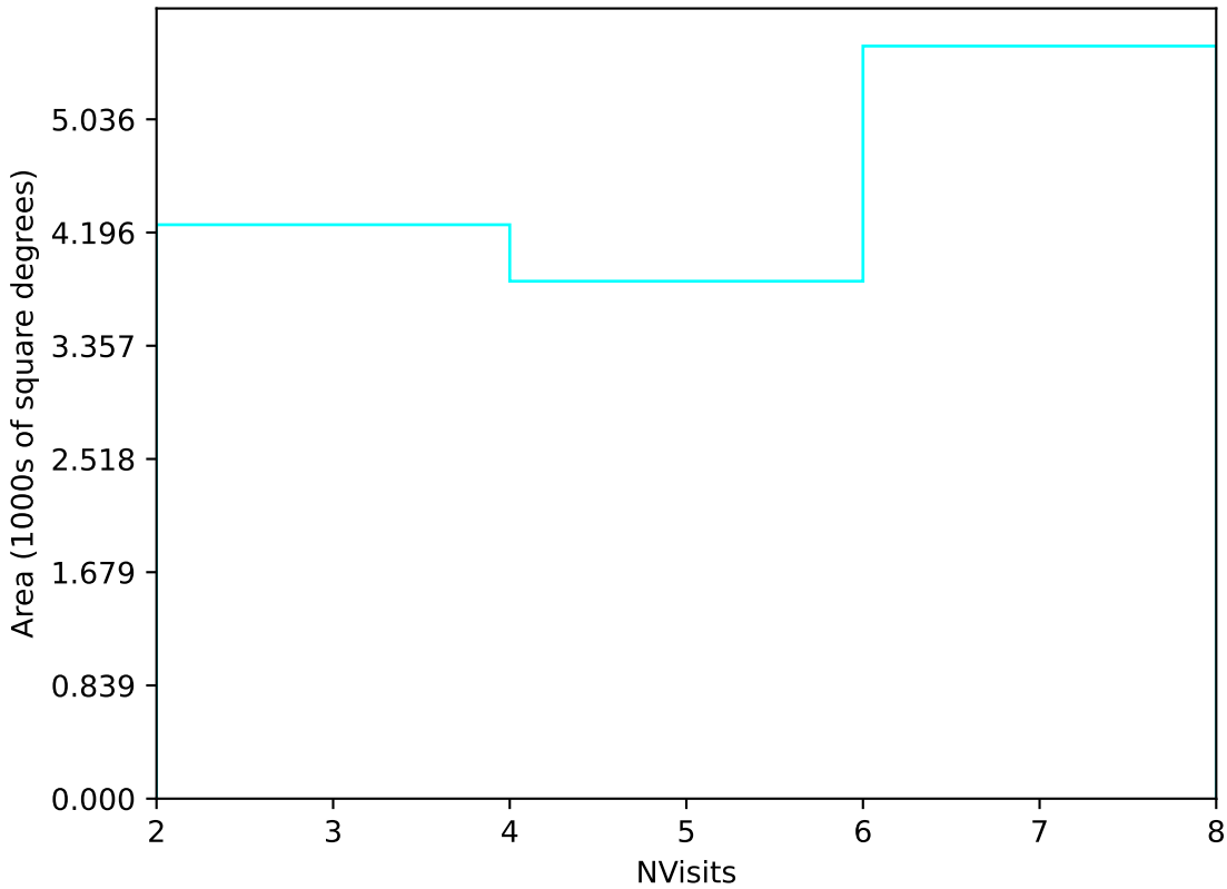
weather_cloudso35v3.4_10yrs Yr 3-4 u band: NVisits
