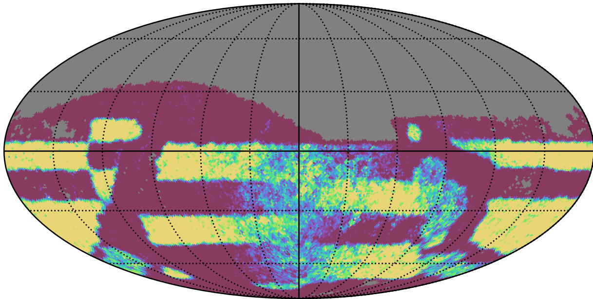
weather_cloudso35v3.4_10yrs Yr 3-4 r band: NVisits
