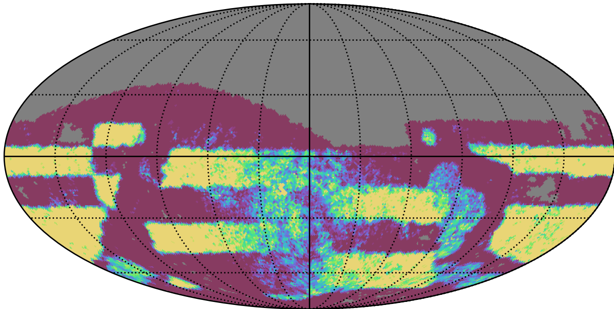
weather_cloudso35v3.4_10yrs Yr 3-4 i band: NVisits
