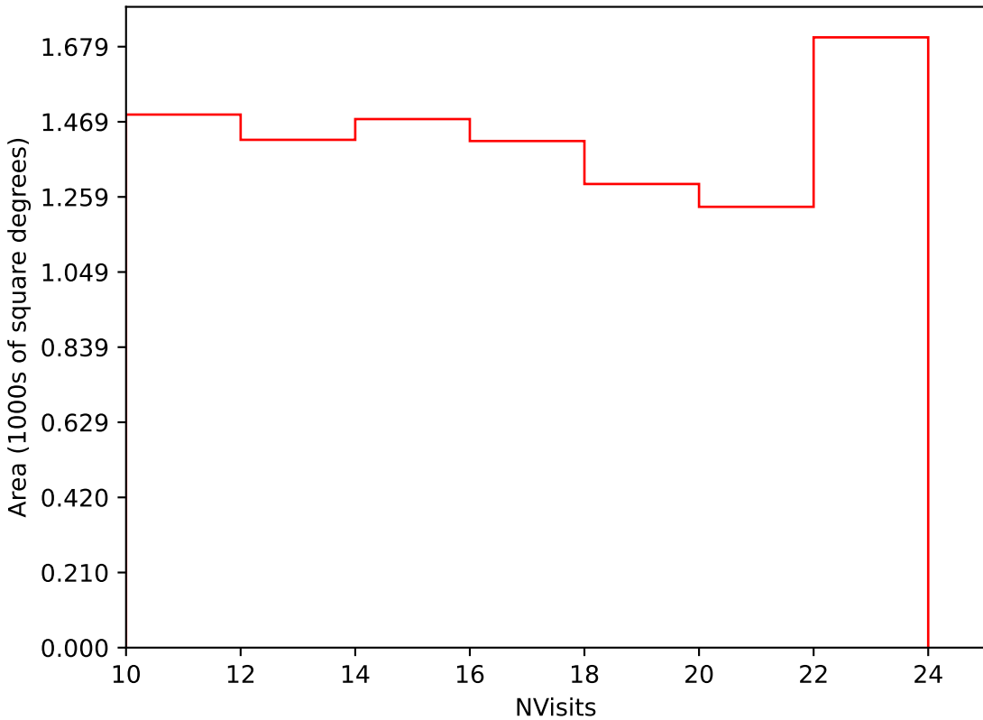
weather_cloudso35v3.4_10yrs Yr 3-4 i band: NVisits
