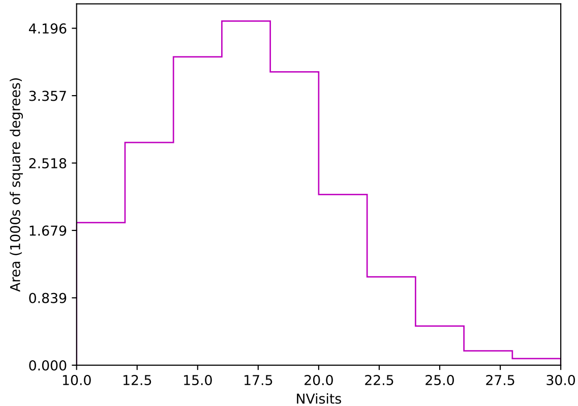
weather_cloudso35v3.4_10yrs Yr 1 z band: NVisits
