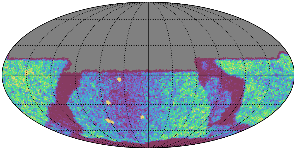
weather_cloudso35v3.4_10yrs Yr 1 y band: NVisits
