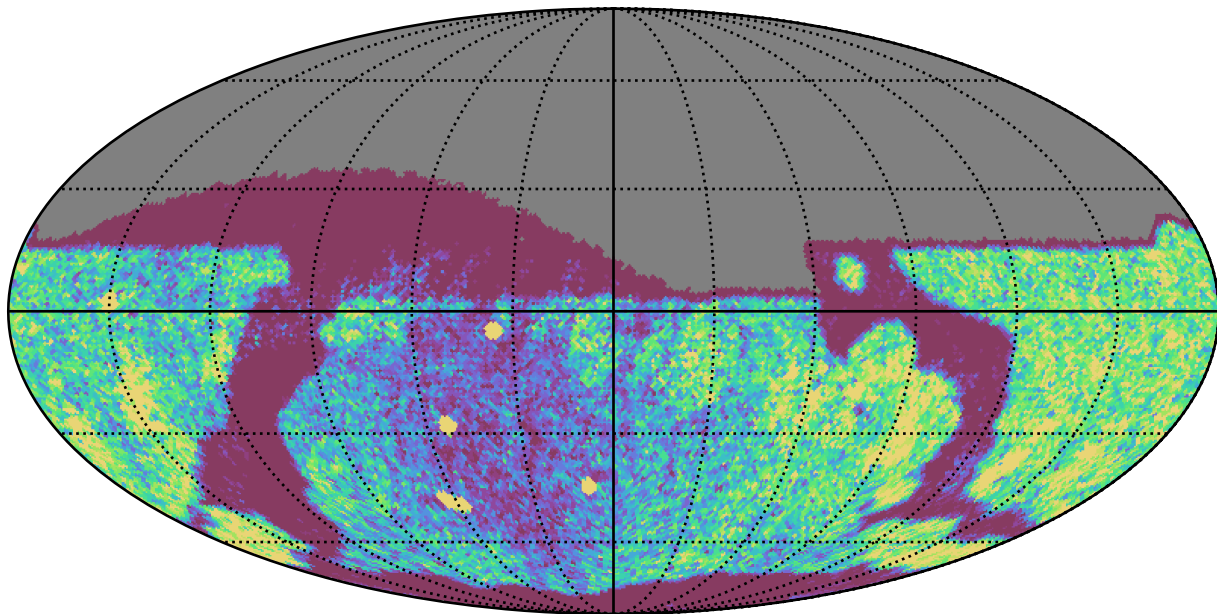
weather_cloudso35v3.4_10yrs Yr 1 r band: NVisits
