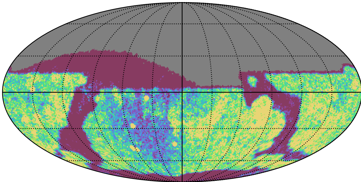
weather_cloudso35v3.4_10yrs Yr 1 i band: NVisits
