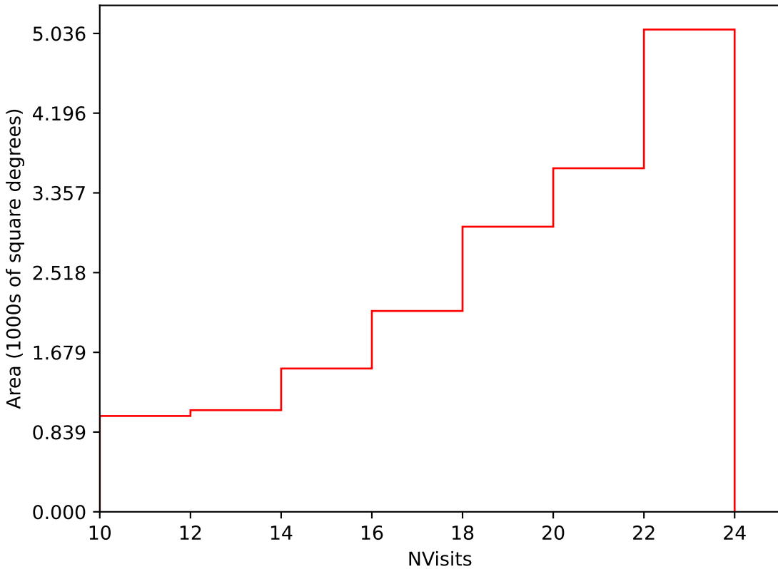
weather_cloudso35v3.4_10yrs Yr 1 i band: NVisits
