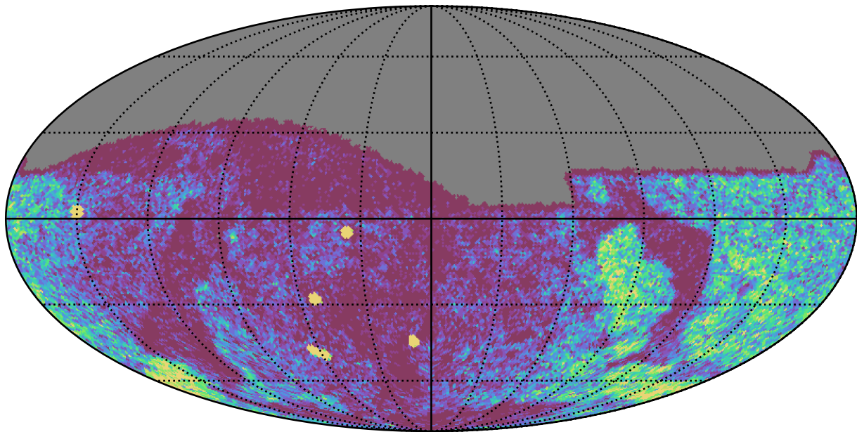
weather_cloudso35v3.4_10yrs Yr 1 g band: NVisits
