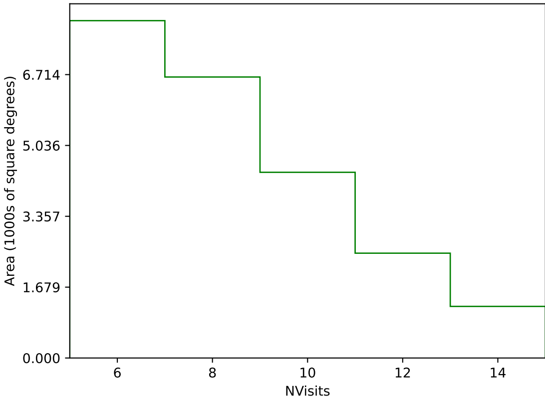
weather_cloudso35v3.4_10yrs Yr 1 g band: NVisits
