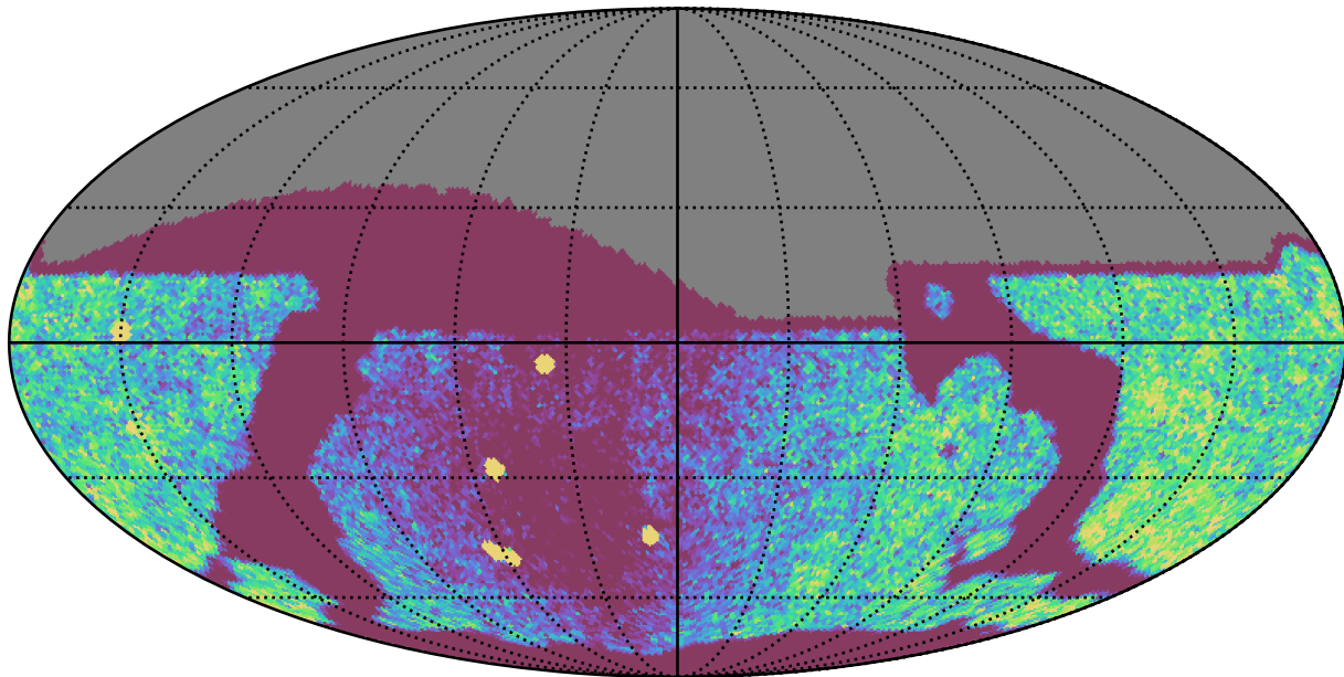
weather_cloudso35v3.4_10yrs Yr 1 all bands: NVisits
