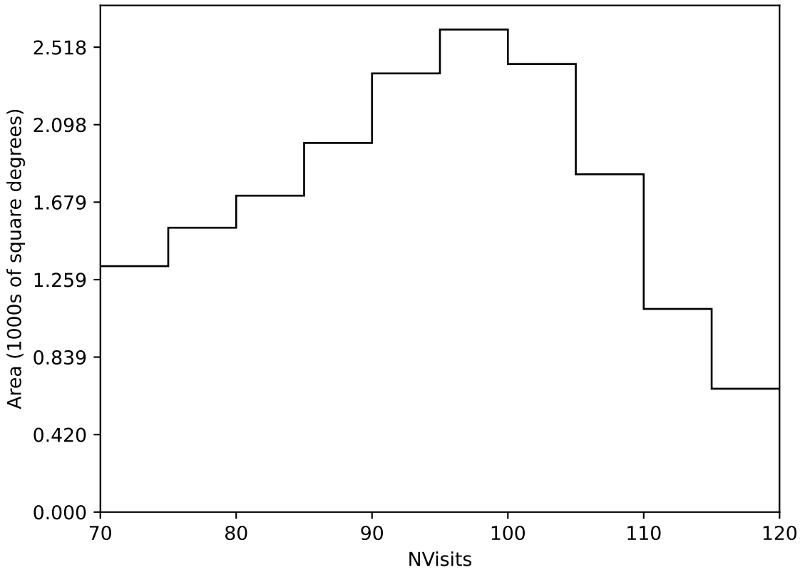
weather_cloudso35v3.4_10yrs Yr 1 all bands: NVisits
