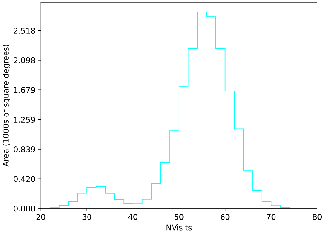
weather_cloudso35v3.4_10yrs WFD u band: NVisits
