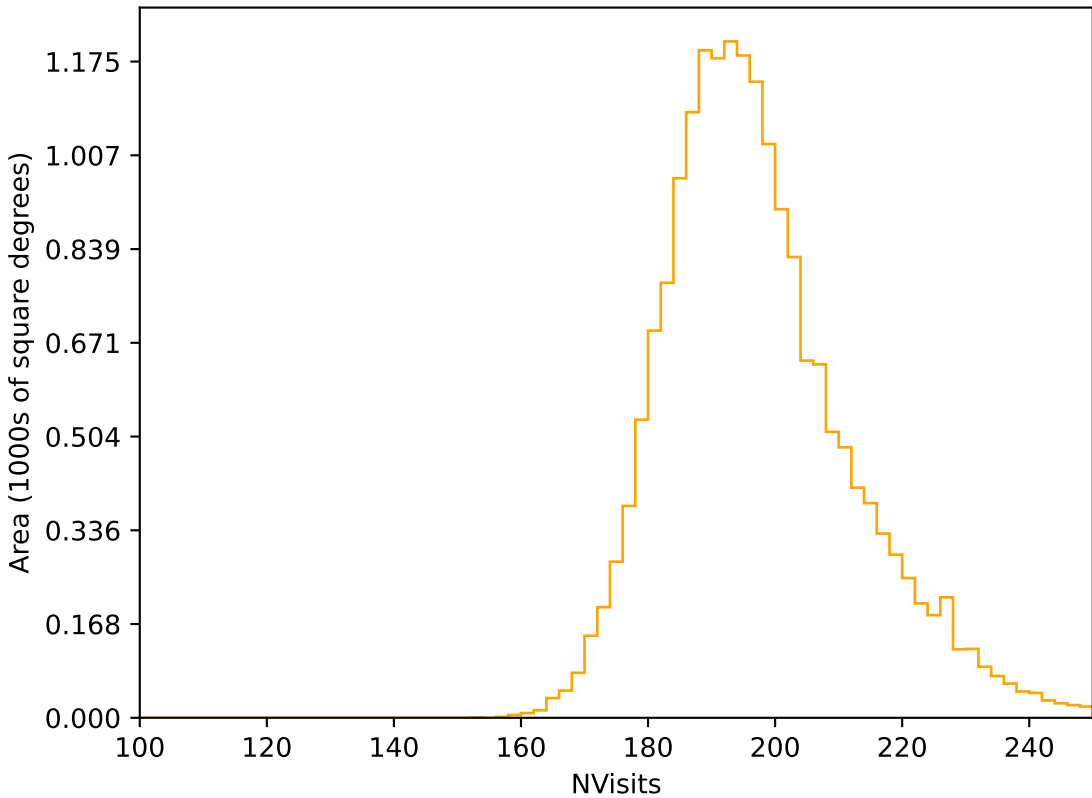
weather_cloudso35v3.4_10yrs WFD r band: NVisits
