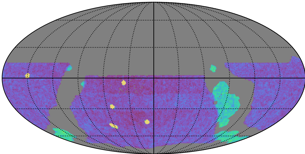
weather_cloudso35v3.4_10yrs WFD g band: NVisits
