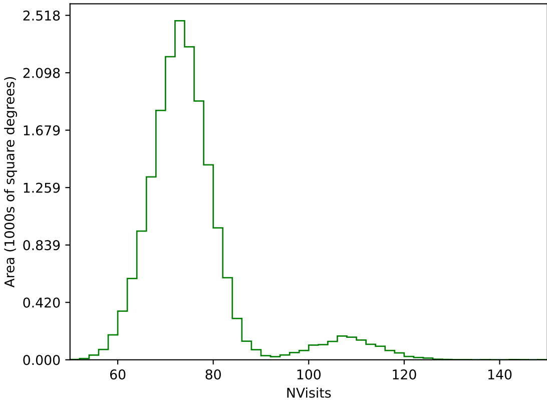
weather_cloudso35v3.4_10yrs WFD g band: NVisits
