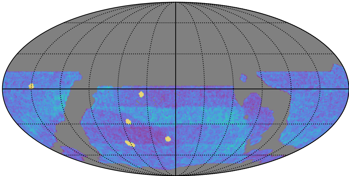
weather_cloudso35v3.4_10yrs WFD all bands: NVisits
