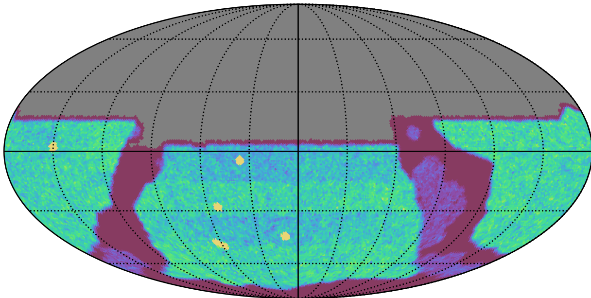
weather_cloudso35v3.4_10yrs All sky u band: NVisits
