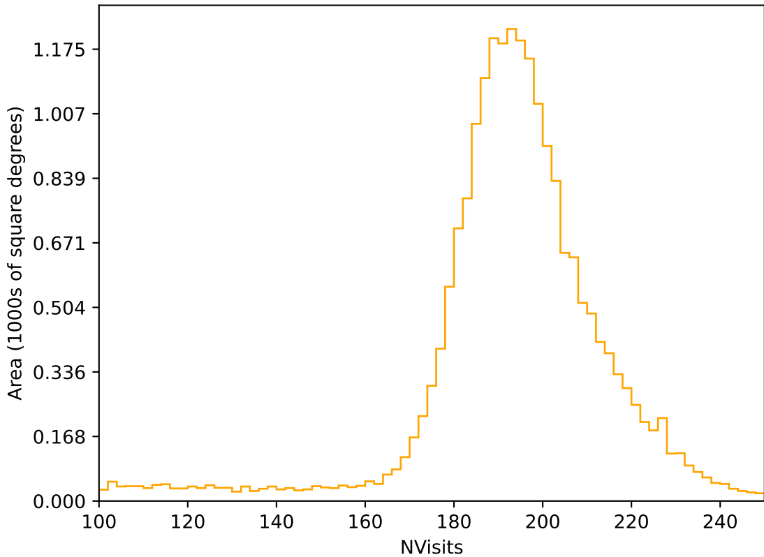
weather_cloudso35v3.4_10yrs All sky r band: NVisits
