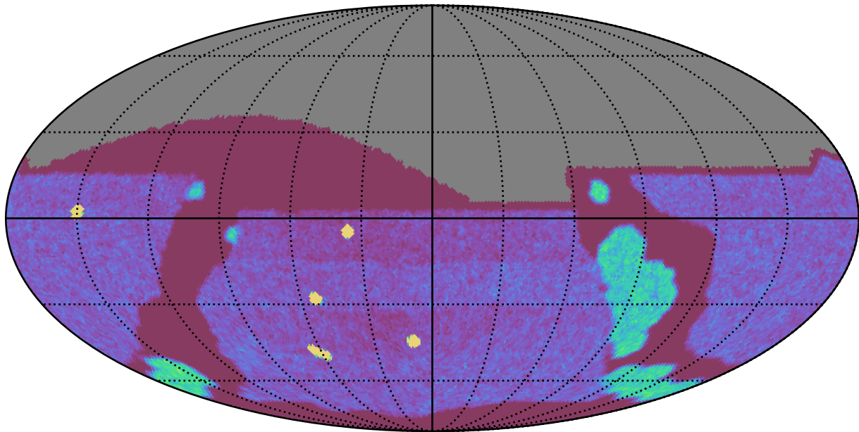
weather_cloudso35v3.4_10yrs All sky g band: NVisits
