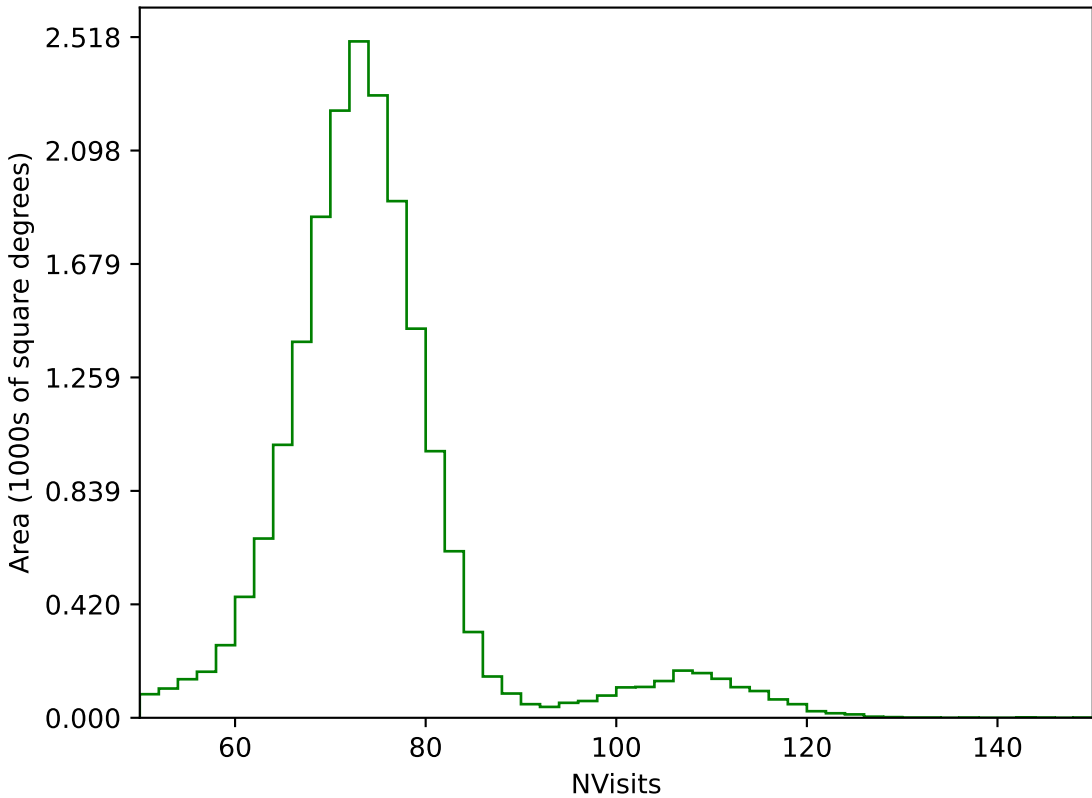
weather_cloudso35v3.4_10yrs All sky g band: NVisits
