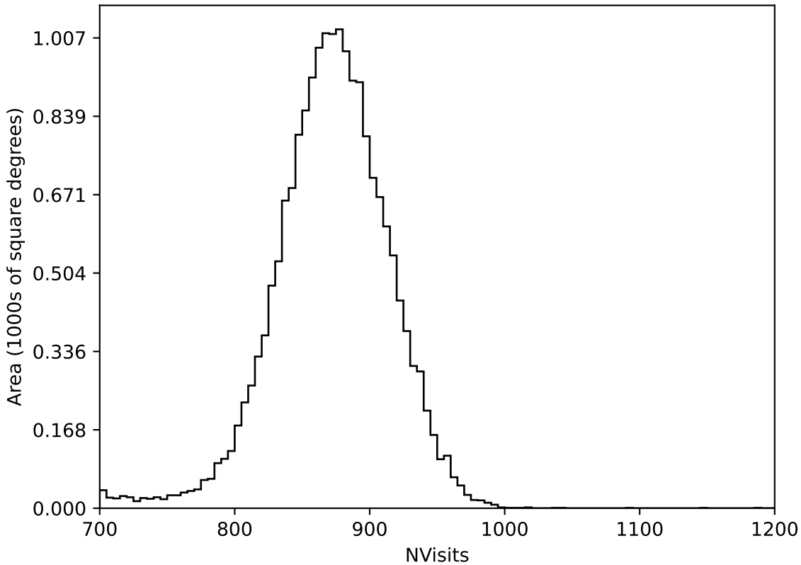
weather_cloudso35v3.4_10yrs All sky all bands: NVisits
