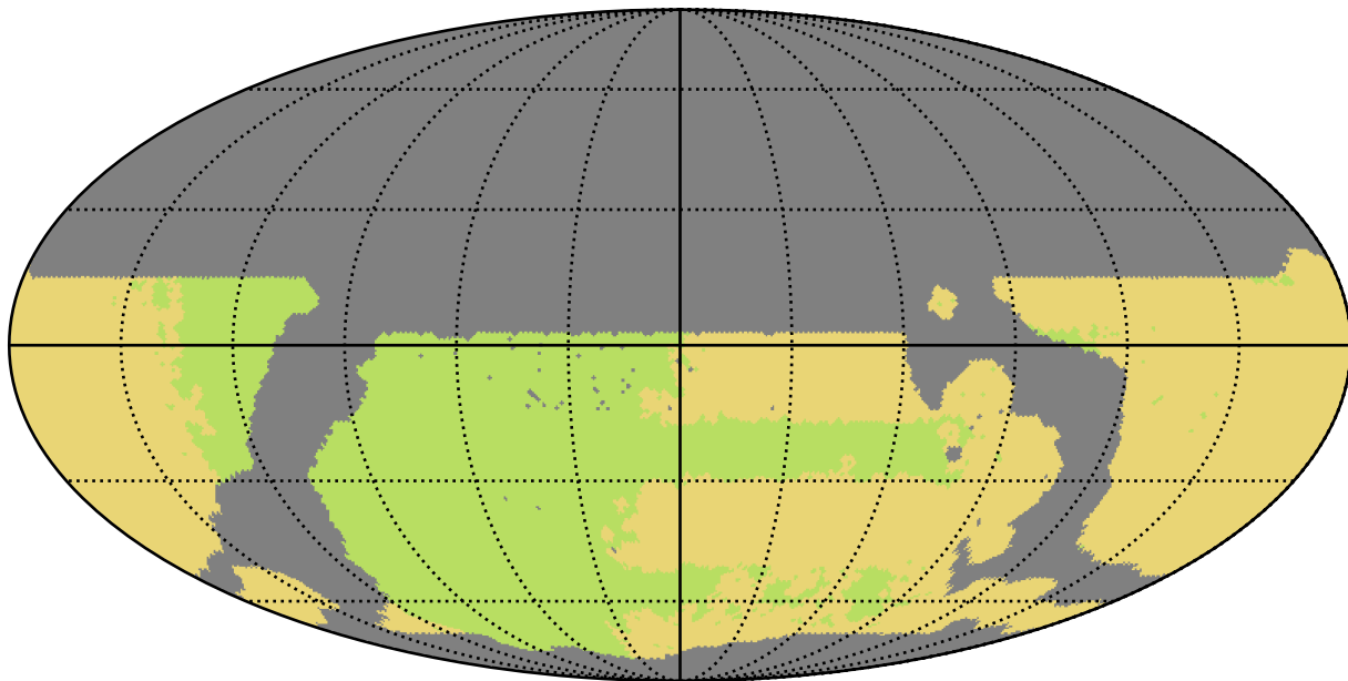
weather_cloudso35v3.4_10yrs WFD all bands: NSeasons
