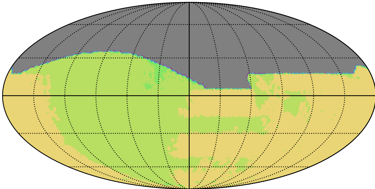
weather_cloudso35v3.4_10yrs All sky all bands: NSeasons
