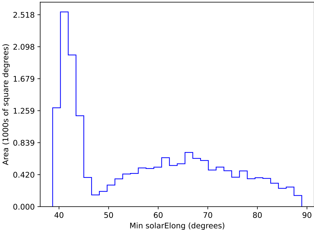
weather_cloudso35v3.4_10yrs WFD r band: Min solarElong
