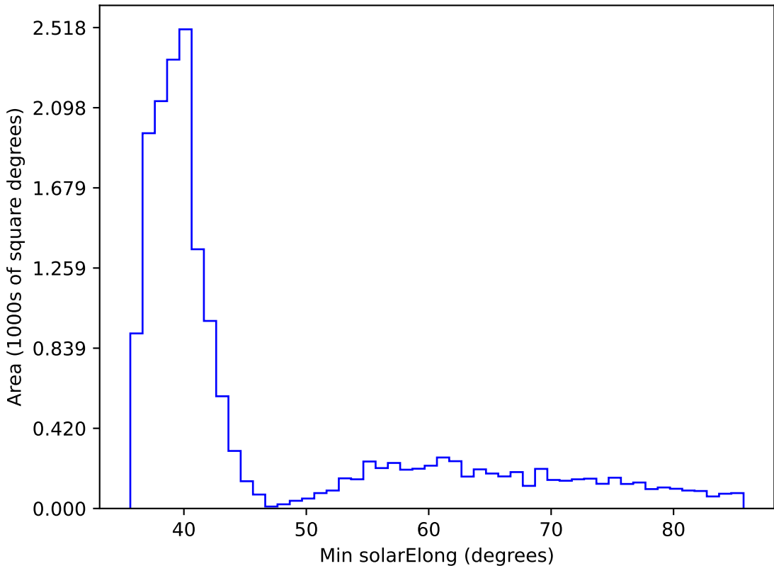
weather_cloudso35v3.4_10yrs WFD all bands: Min solarElong
