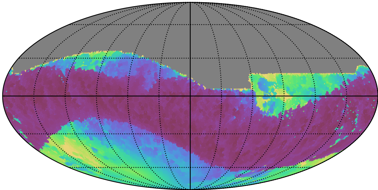
weather_cloudso35v3.4_10yrs All sky z band: Min solarElong
