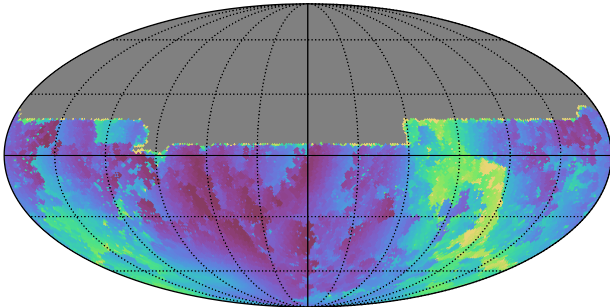
weather_cloudso35v3.4_10yrs All sky u band: Min solarElong
