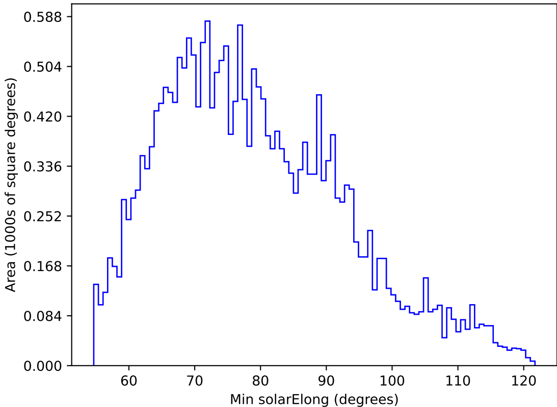
weather_cloudso35v3.4_10yrs All sky u band: Min solarElong
