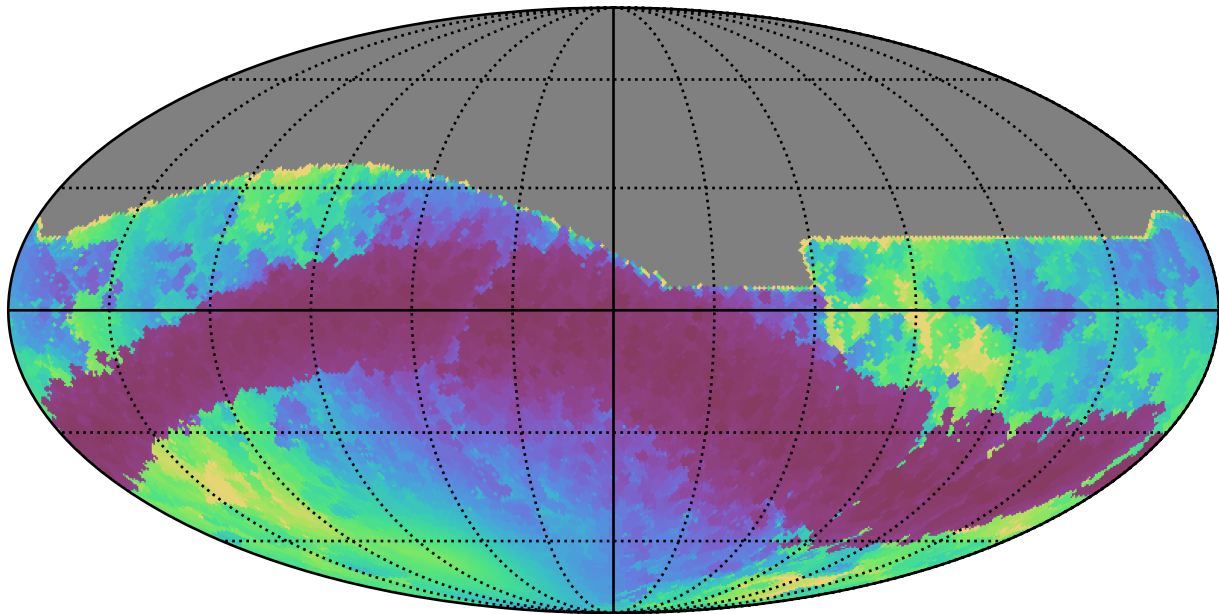
weather_cloudso35v3.4_10yrs All sky r band: Min solarElong
