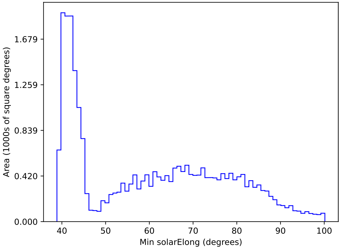
weather_cloudso35v3.4_10yrs All sky r band: Min solarElong
