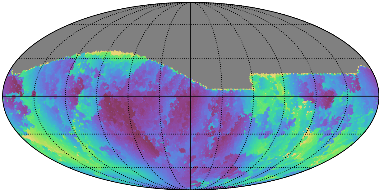
weather_cloudso35v3.4_10yrs All sky g band: Min solarElong
