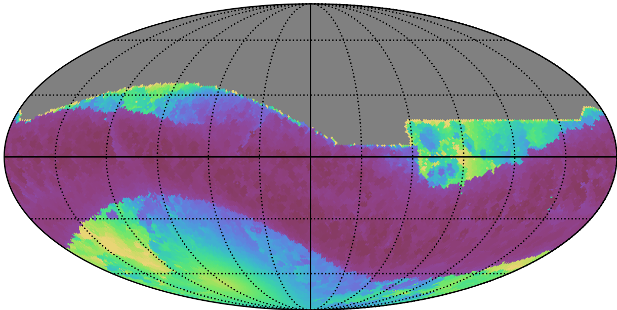
weather_cloudso35v3.4_10yrs All sky all bands: Min solarElong
