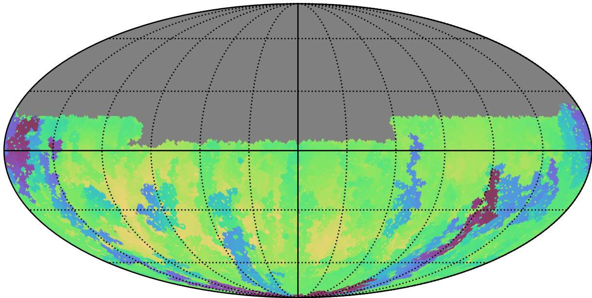
weather_cloudso35v3.4_10yrs Yr 1 u band: Min skyBrightness
