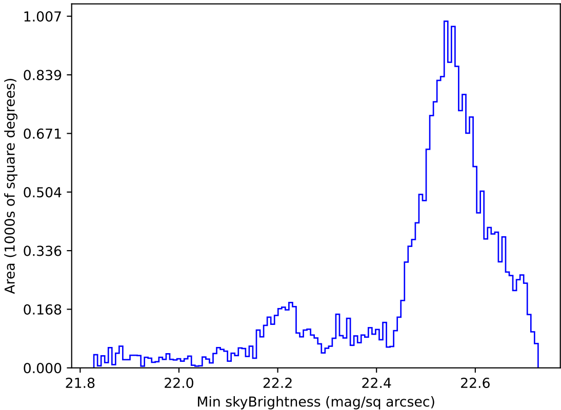
weather_cloudso35v3.4_10yrs Yr 1 u band: Min skyBrightness
