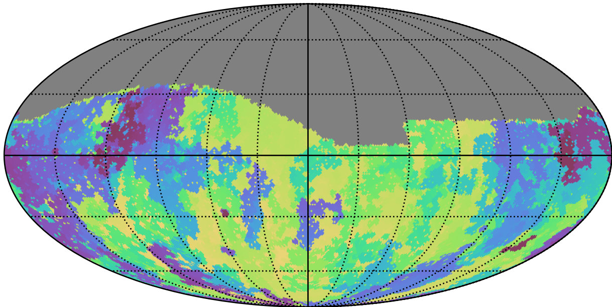
weather_cloudso35v3.4_10yrs Yr 1 g band: Min skyBrightness
