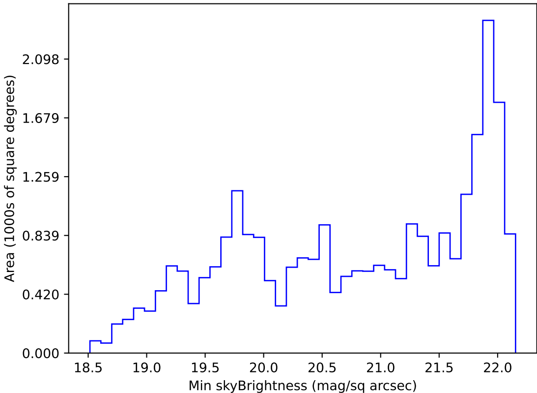
weather_cloudso35v3.4_10yrs Yr 1 g band: Min skyBrightness
