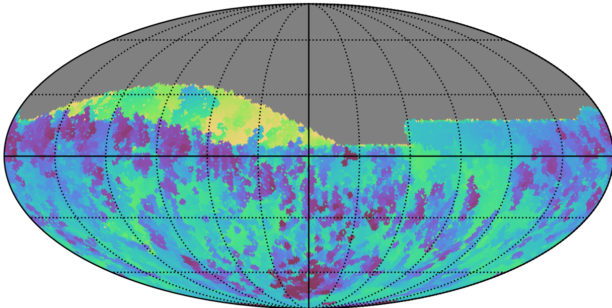
weather_cloudso35v3.4_10yrs Yr 1 all bands: Min skyBrightness
