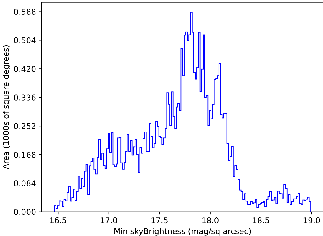
weather_cloudso35v3.4_10yrs Yr 1 all bands: Min skyBrightness
