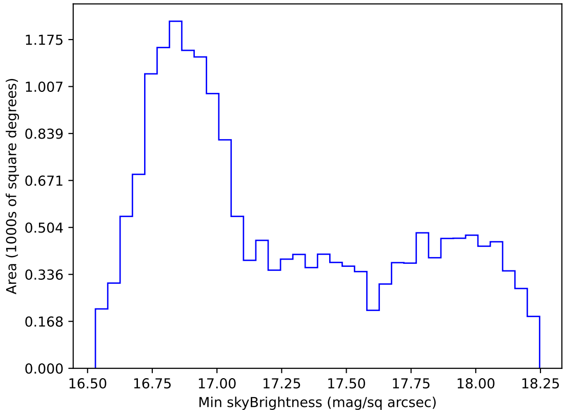
weather_cloudso35v3.4_10yrs WFD z band: Min skyBrightness
