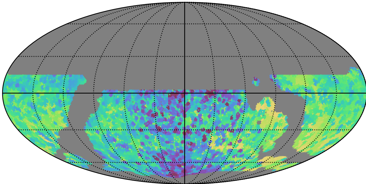
weather_cloudso35v3.4_10yrs WFD y band: Min skyBrightness
