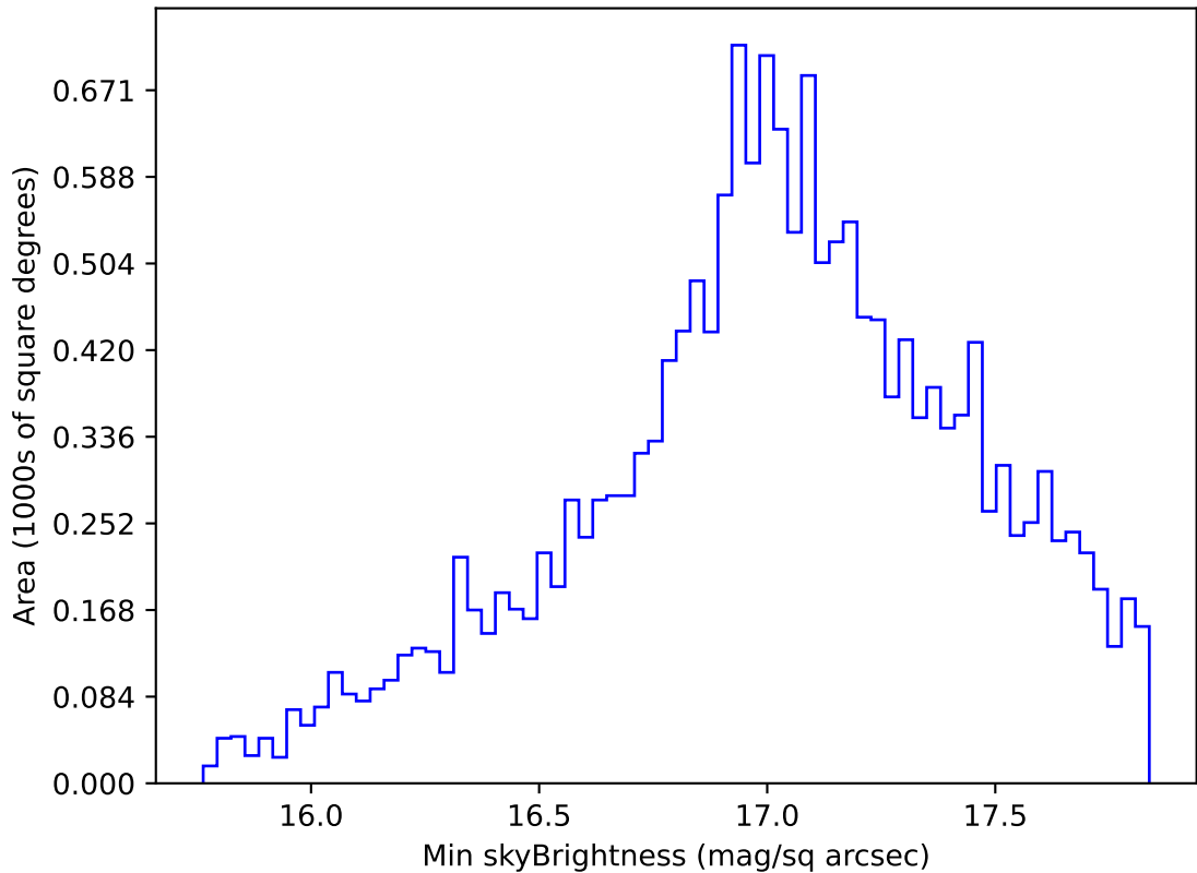
weather_cloudso35v3.4_10yrs WFD y band: Min skyBrightness
