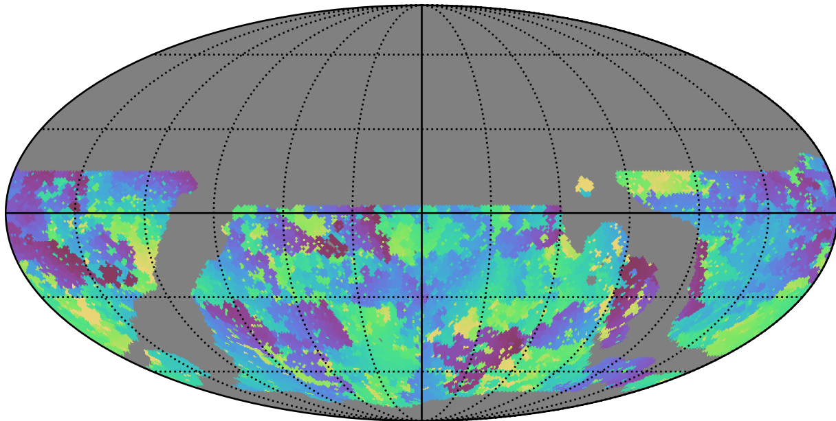
weather_cloudso35v3.4_10yrs WFD u band: Min skyBrightness
